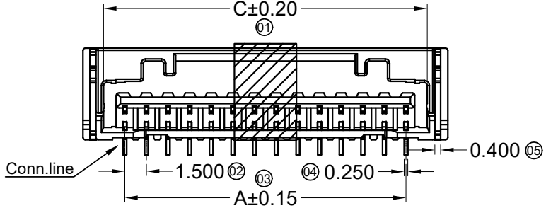
06P-15P Single Hole
