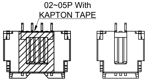
03P-05P Single Hole Scale 1:1
