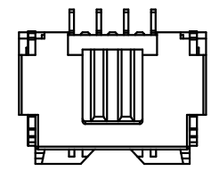
03P-05P Single Hole Scale 1:1
