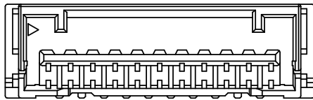
11 PIN
